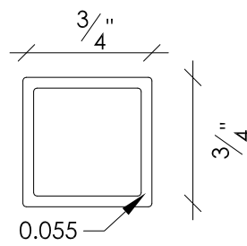
WALL PICKET TOPVIEW SCALE: 1' = 1'-0"
