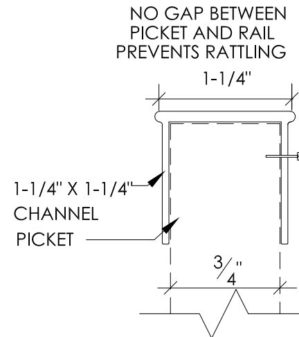
PICKET FASTENED TO CHANNEL DETAIL SCALE: 1' = 1'-0"
