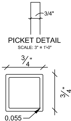
WALL PICKET TOPVIEW SCALE: 1' = 1'-0"
