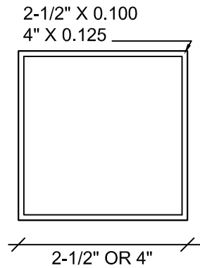
WALL POST TOP VIEW SCALE: 6" = 1'-0"
