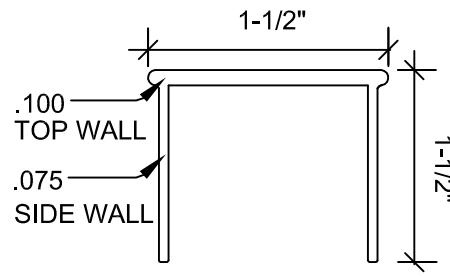
RAIL DETAIL SCALE: 1' = 1'-0"
